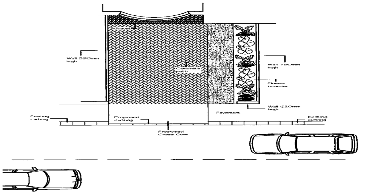
Proposed Layout
